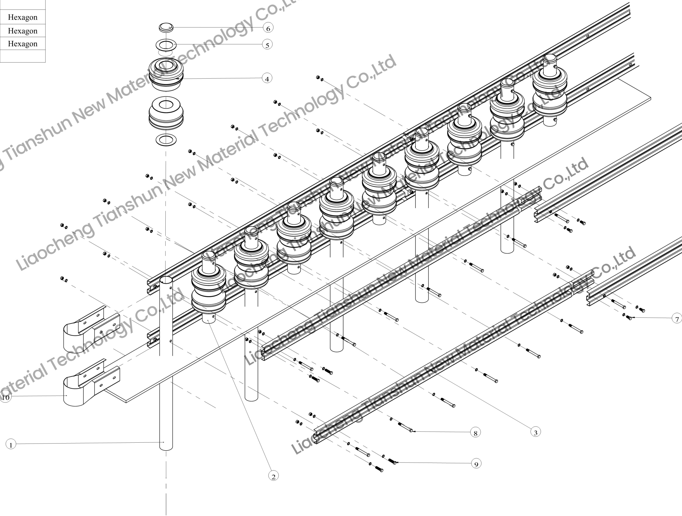
EXPLOSIVE VIEW 1:25
